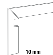
BATTISCOPIA SCALA CON SCASSO DX / SX INTERLOCKING TREAD SKIRTING DX / SX 7,5x60x60 - 2 15/16 "x23 5/8 "x23 5/8 " Pcs. Box. 2 - ML x Box 1,20 BB4F8RD / BB4F8RS SLATE GREY NAT. RETT. ● 36
