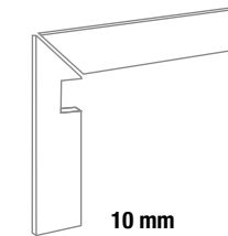
BATTISCOPIA SCALA CON SCASSO DX / SX INTERLOCKING TREAD SKIRTING DX / SX 7,5x60x60 - 2 15/16 "x23 5/8 "x23 5/8 " Pcs. Box. 2 - ML x Box 1,20 BB4F7RD / BB4F7RS GRANITE STONE NAT. RETT. ● 36
